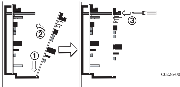
Figure 6b. Installation of XP10-M module in front chassis position:
