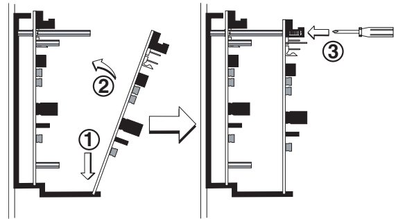
Figure 6b: Installation of XP6-C module in front chassis position
