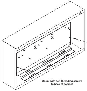
Figure 4: Mounting the CHS-6 chassis
