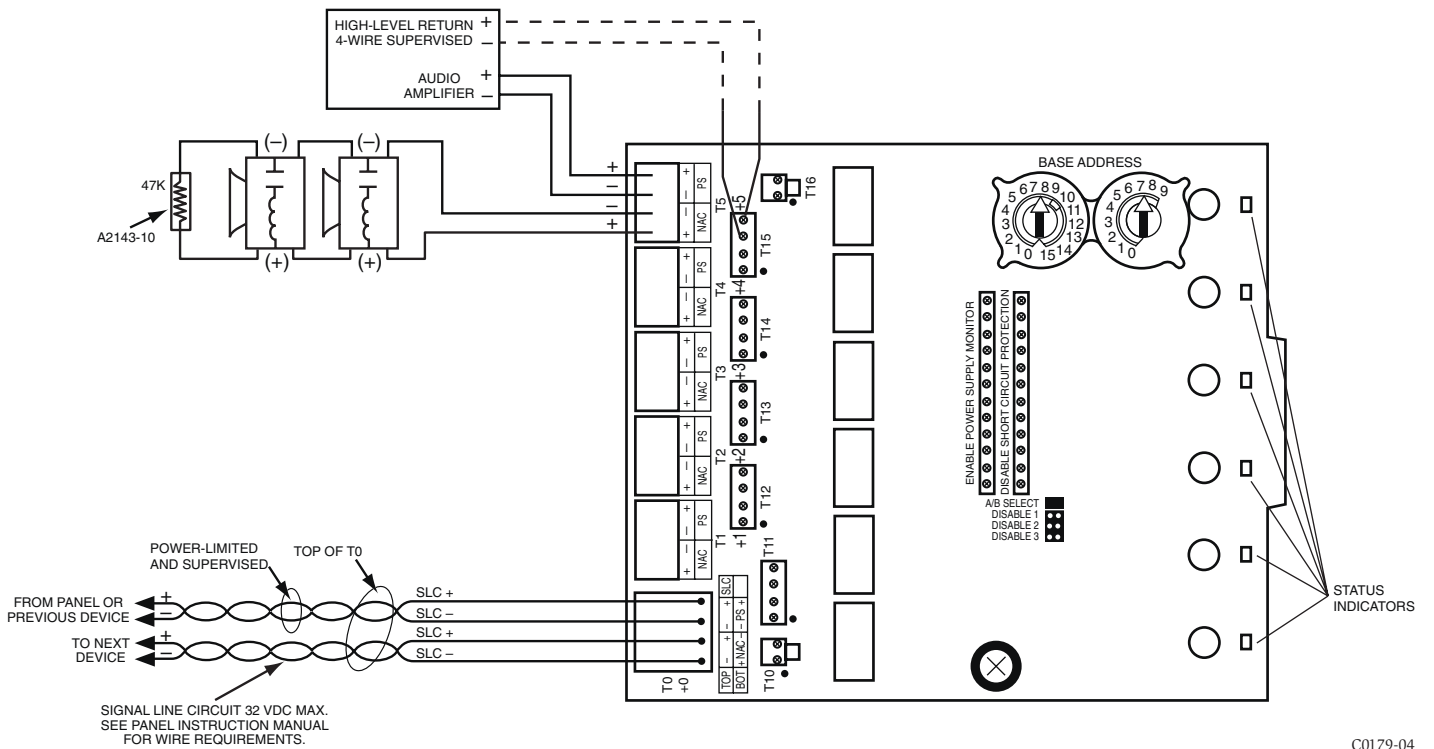
Figure 13: Example of Class B, Style Y Audio NAC configuration.
