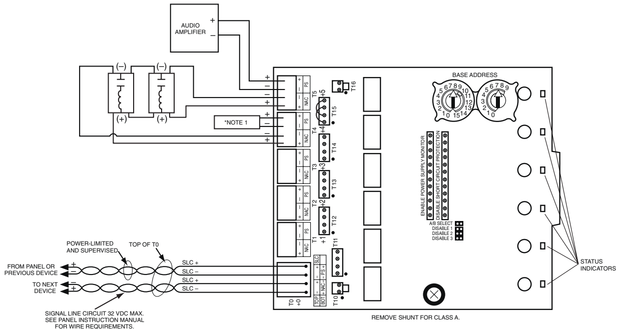
Figure 14: Example of Class A, Style Z Audio NAC configuration.
