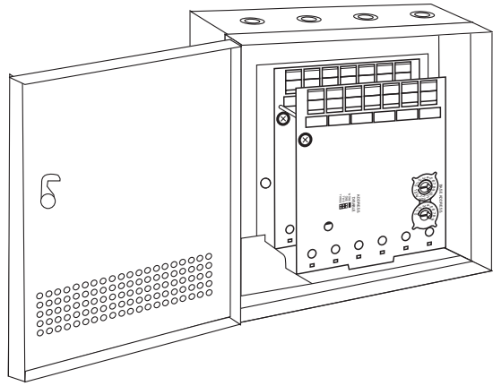
Figure 2: BB-XP Cabinet
