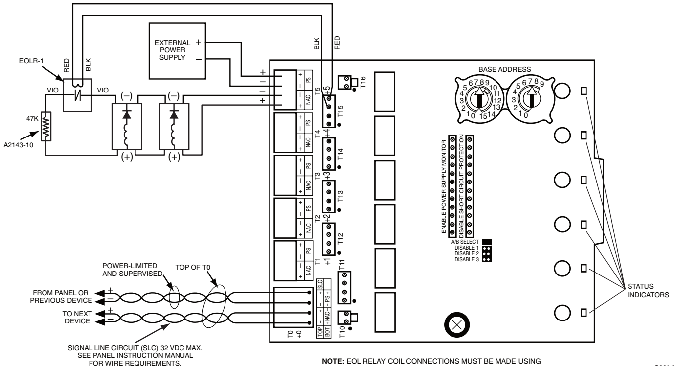
Figure 9: Example of Class B, Style Y NAC configuration with a single supply dedicated to a single NAC.
