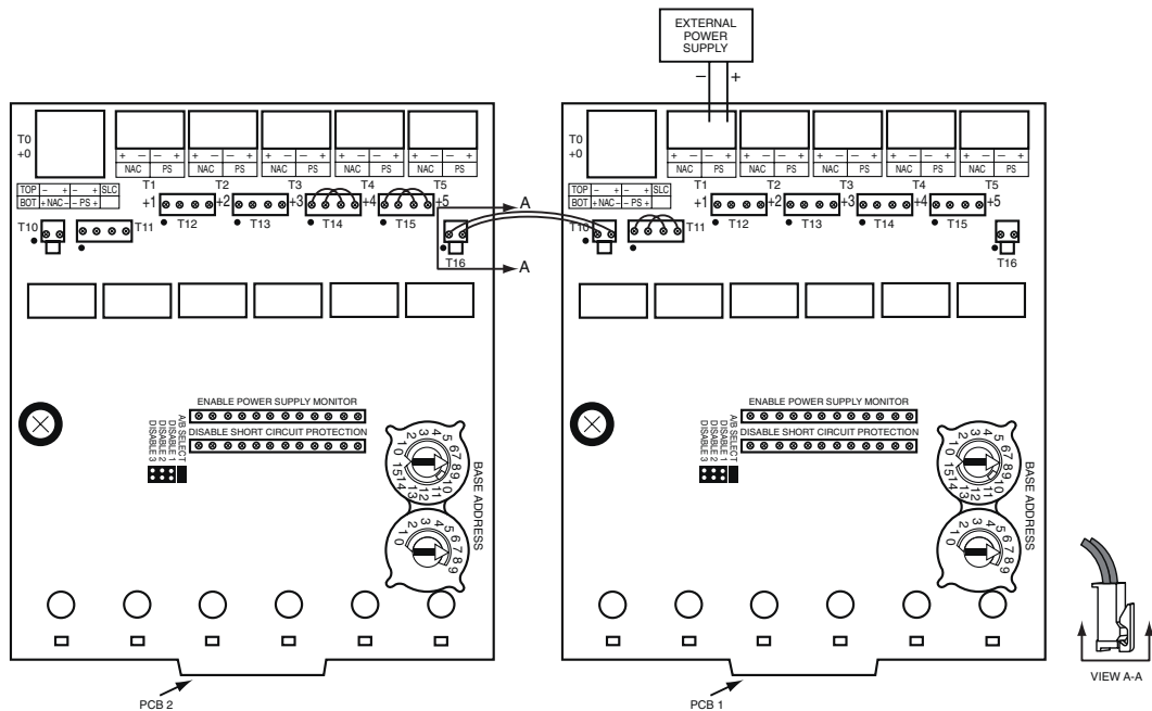
Figure 15: Example of multiple boards sharing same external supply. Supply is shared by NACs +0 and +1 (on PCB 1) as well as +3, +4, and +5 (on PCB 2). Refer to figures 9–12 for typical NAC wiring. Make certain lip on long power supply jumper engages retaining tab on T10 or T16 as shown in View A-A.
