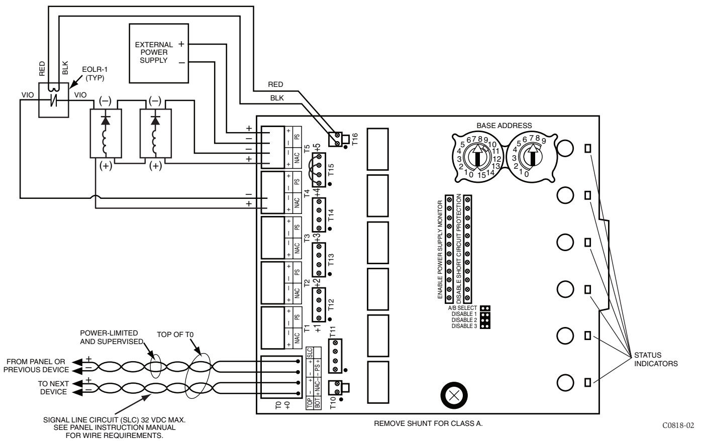
Figure 11: Example of Class A, Style Z NAC configuration with a single supply dedicated to a single NAC.
