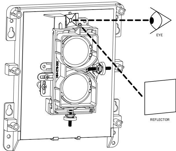
Figure 12. Coarse Alignment Procedure
