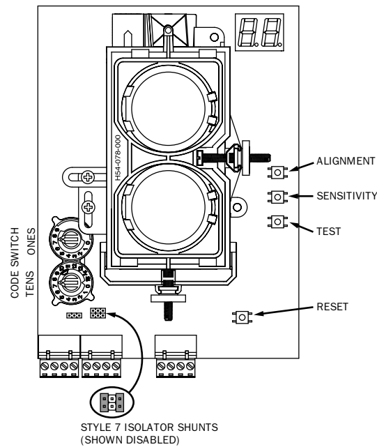
Figure 10. Switch Locations
