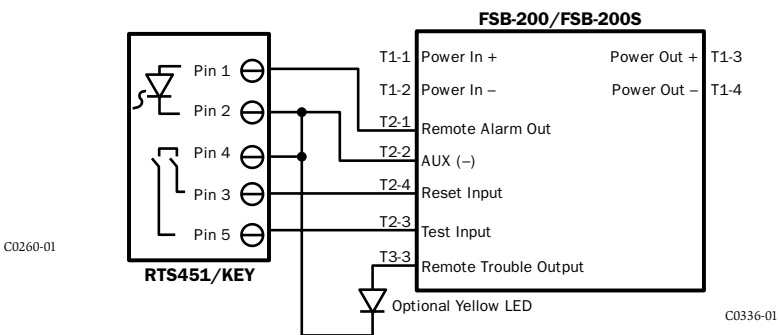
Figure 9. Wiring Diagram (RTS451)
