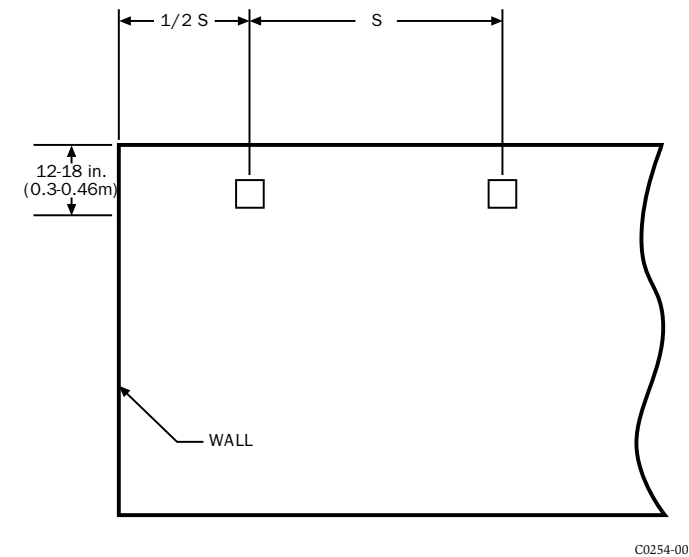
Figure 1. Spacing for smooth ceiling (side view):
