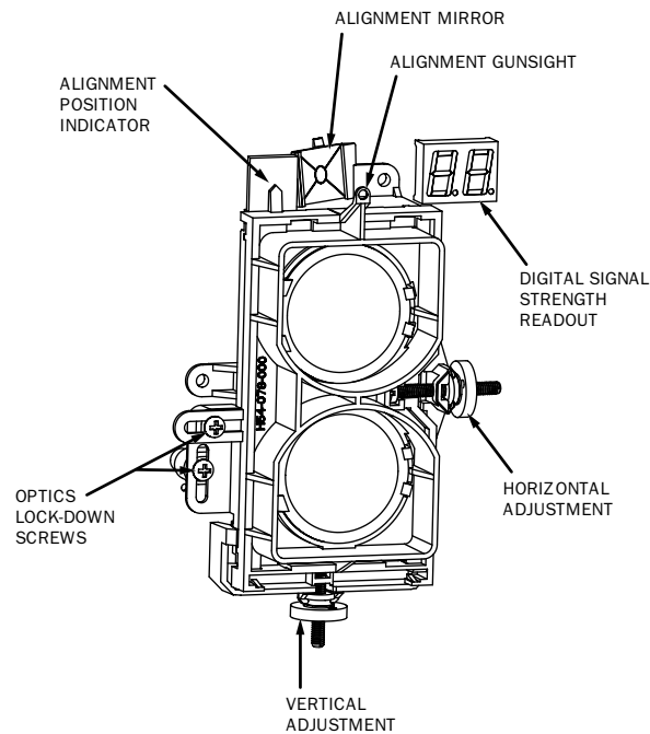
Figure 11. Alignment Adjustment Locations
